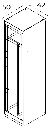
ref. T401M1PSE
